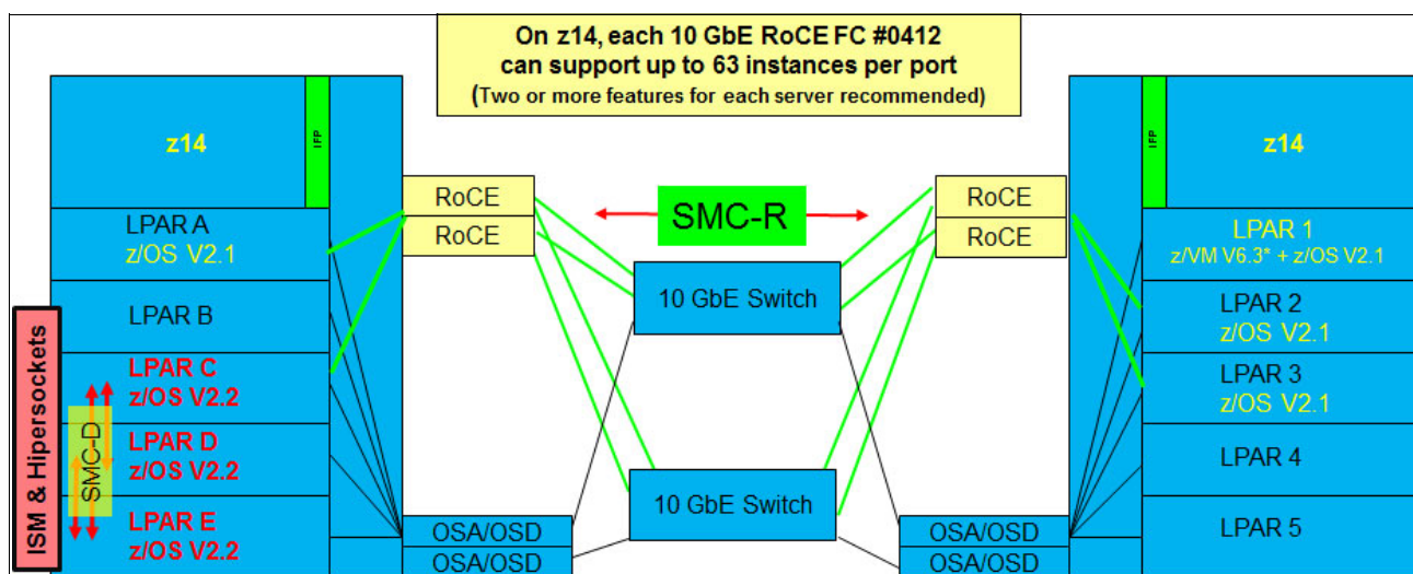
Figure D-5 10GbE RoCE Express sample configuration
