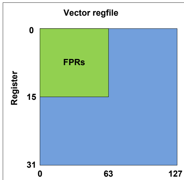
Figure 3-8 Floating point registers overlaid by vector registers
