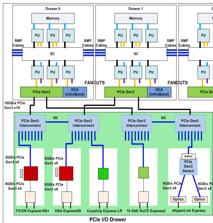
Figure 2-24 Redundant I/O interconnect for PCIe I/O drawer
