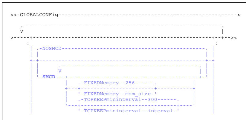
Figure D-19 SMCD parameter in GLOBALCONFIG
