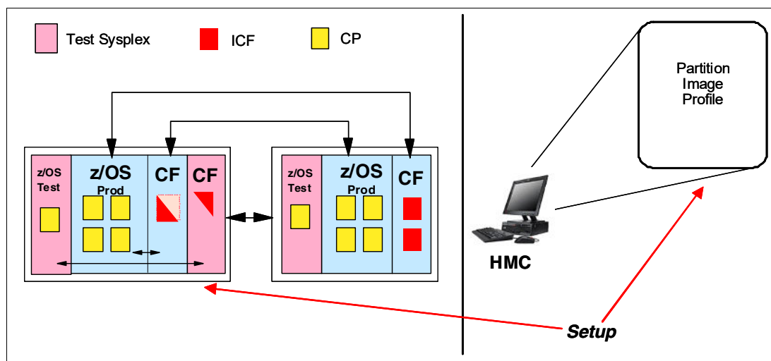
Figure 3-12 ICF options - shared ICFs
