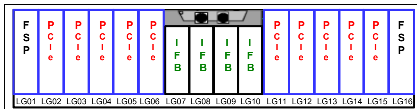
Figure 2-7 z13 CPC drawer front view
