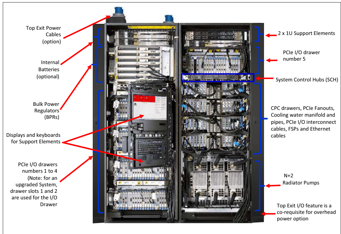
Figure 2-2 z13 internal, front view: Air-cooled platform with five PCIe I/O drawers
