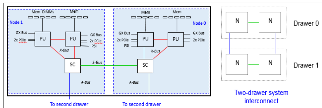
Figure 3-3 z13s CPC drawer interconnect topology (two CPC drawers)
