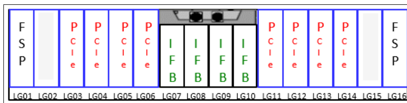
Figure 3-7 N20 CPC drawer front view
