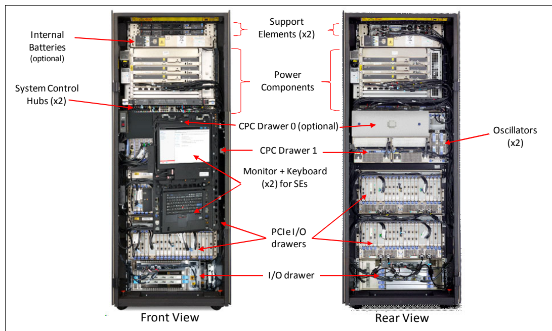
Figure 3-2 z13s internal front and rear view: Air-cooled platform with two PCIe drawers and one I/O drawer
