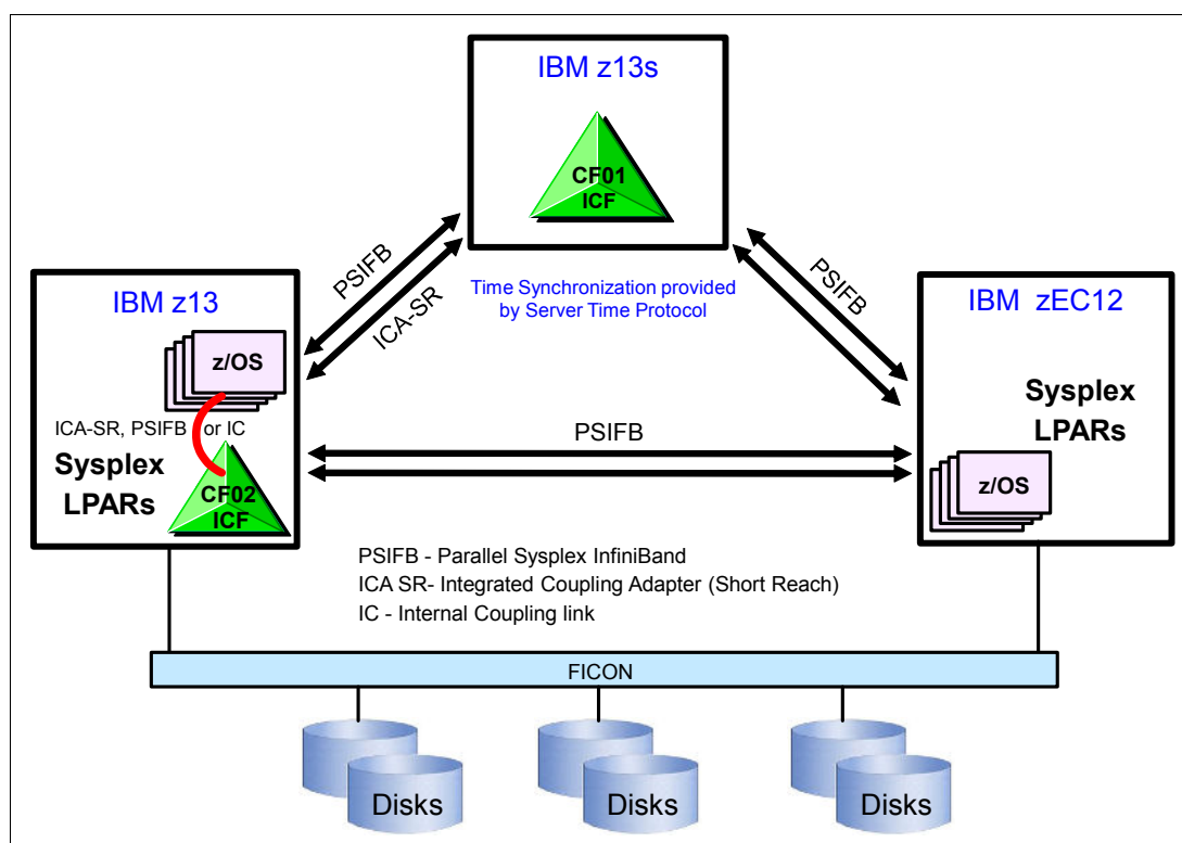
Figure 5-4 Sysplex hardware overview
