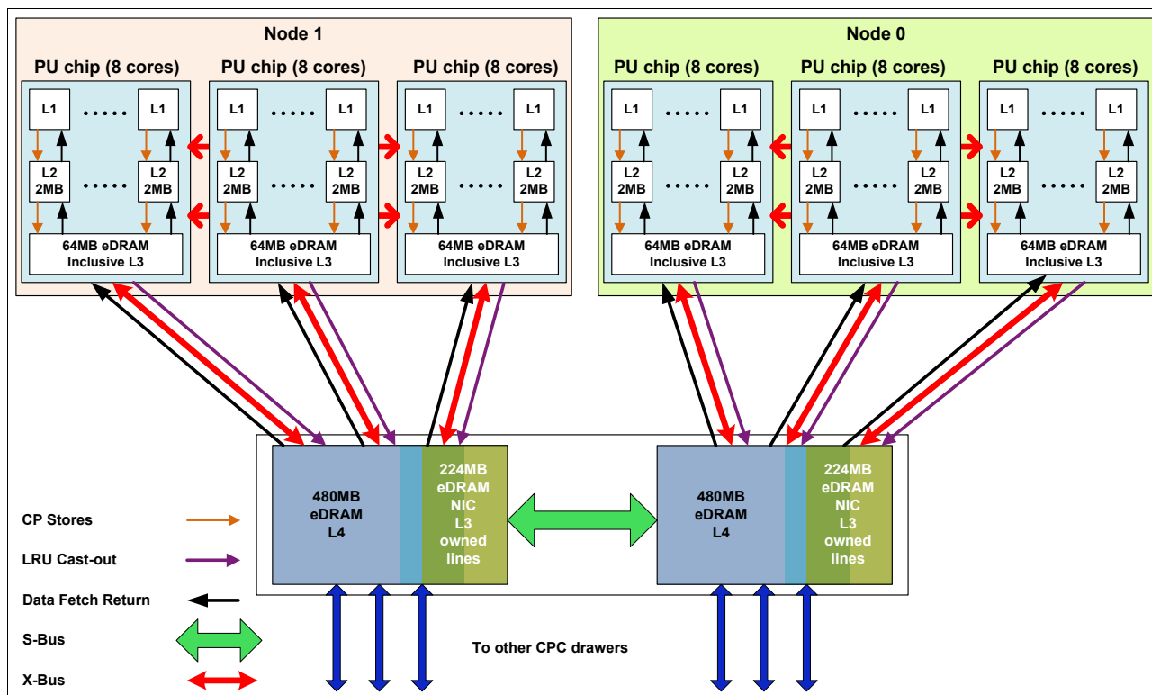
Figure 2-5 z13 CPC drawer chips and cache structure
