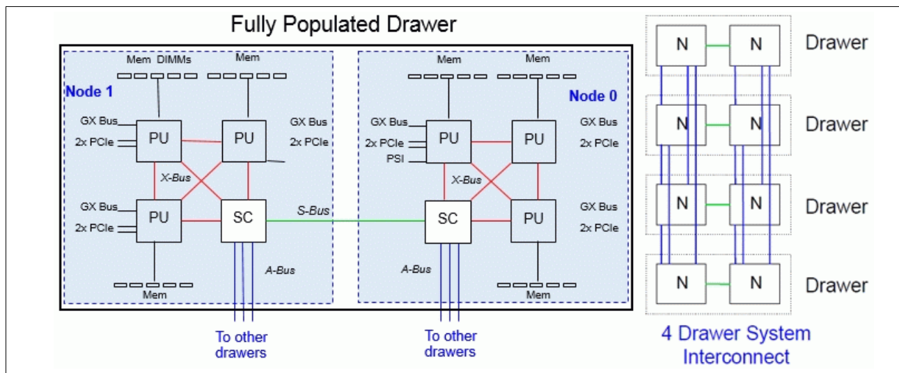
Figure 2-4 z13 CPC drawer communication topology
