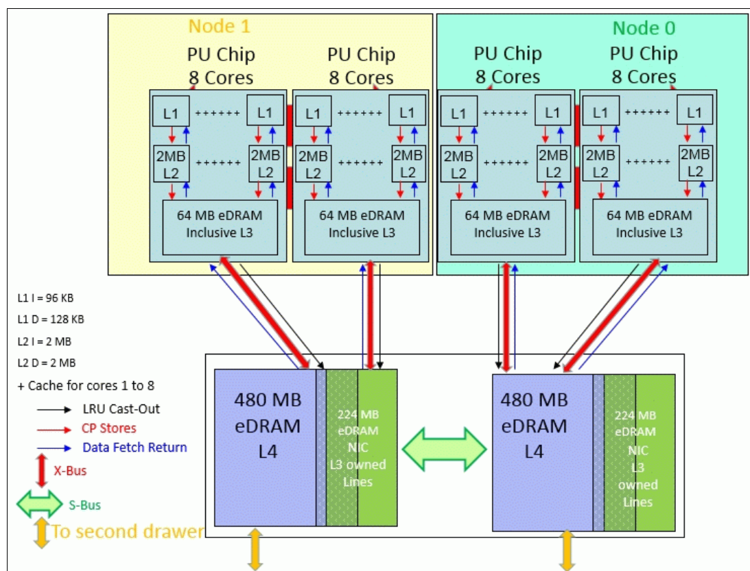
Figure 3-4 z13s CPC drawer chips and cache structure
