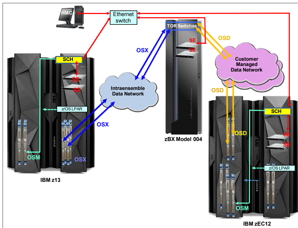
Figure 4-1 IEDN and client-managed data networks in an ensemble
