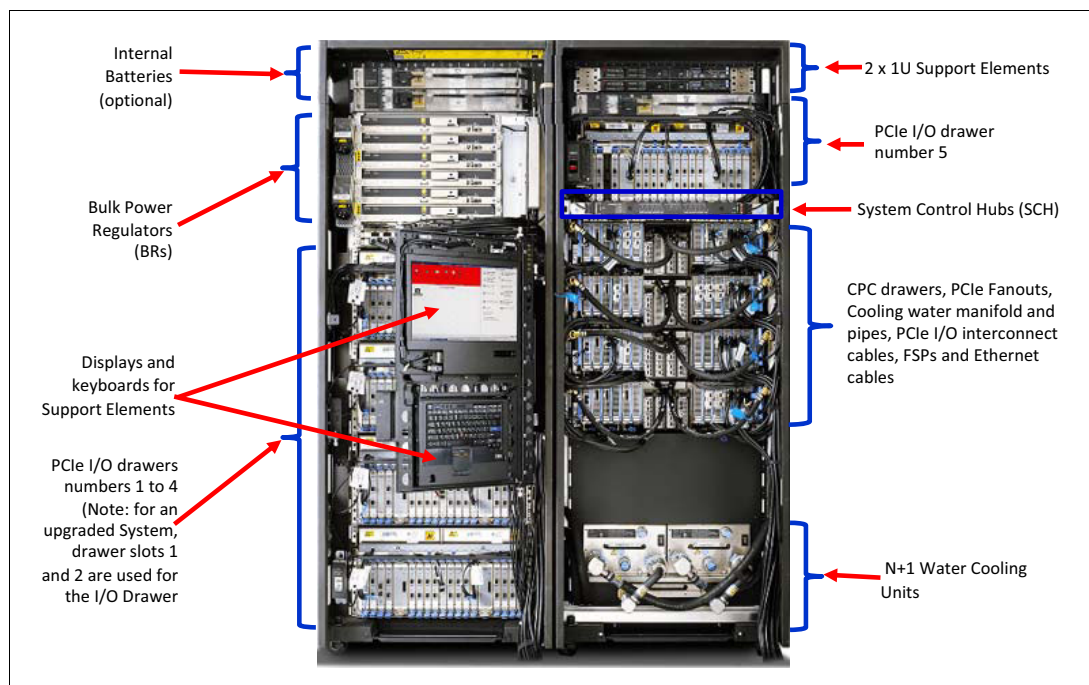
Figure 2-3 z13 internal, front view: Water-cooled platform with five PCIe I/O drawers
