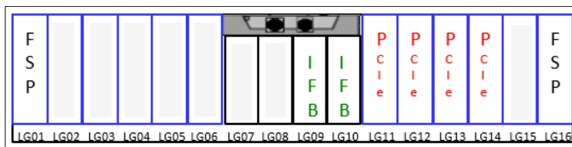
Figure 3-6 N10 CPC drawer front view
