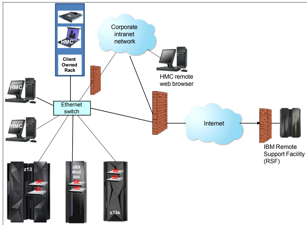
Figure 4-3 HMC and SE connectivity
