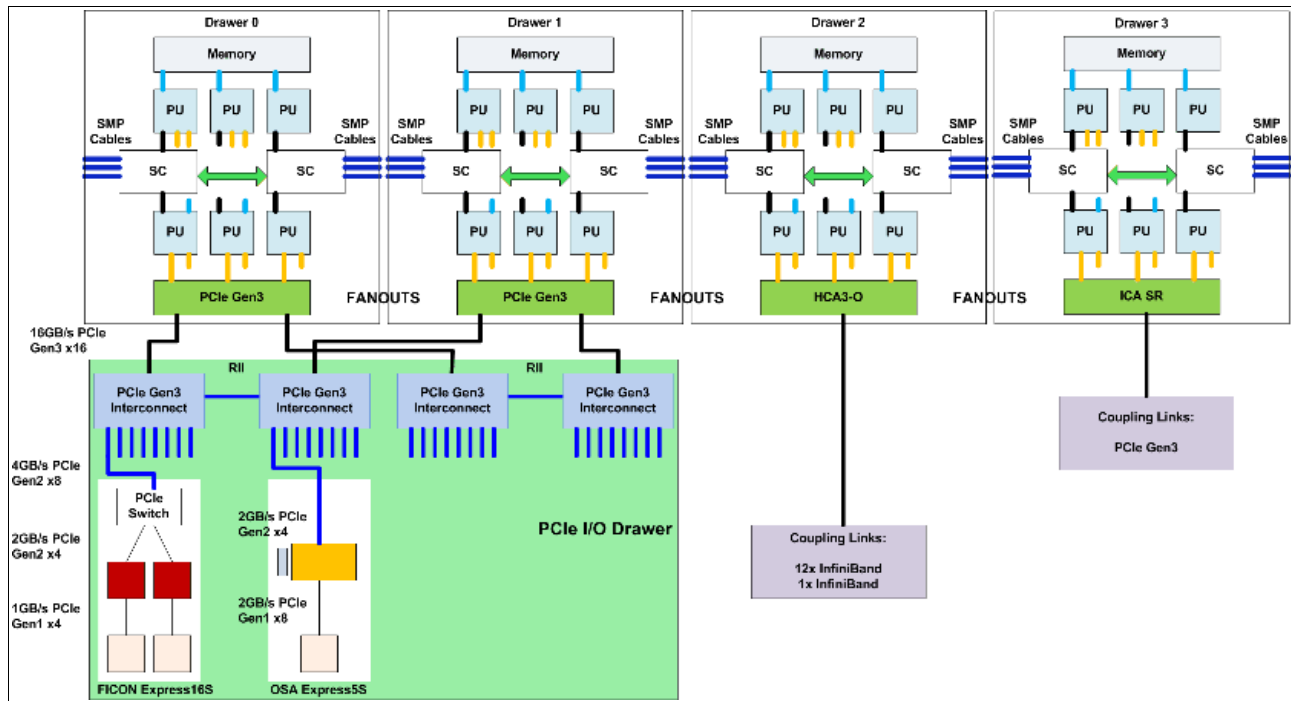
Figure 2-6 z13 I/O system structure
