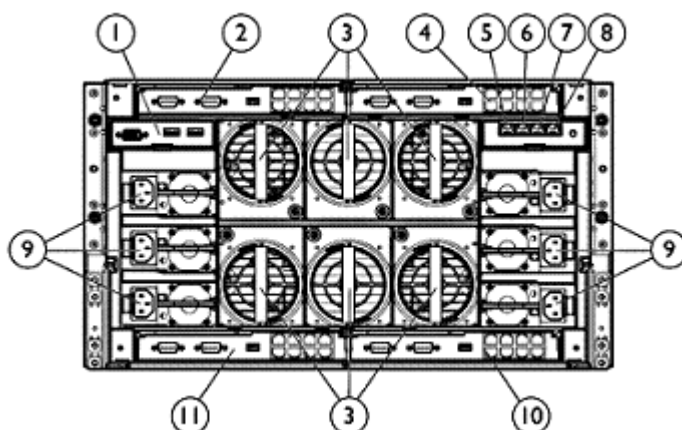
HP BladeSystem c3000 Platinum Enclosure - Rack - Rear View
