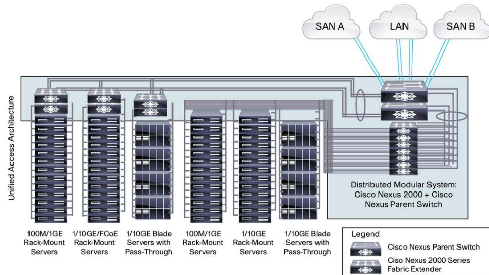
Figure 13. Sample Unified Access Deployment Scenario Supporting Up to 1152 1 Gigabit Ethernet Servers or Up to 768 10 Gigabit Ethernet Servers with a Single Pair of Access-Layer Switches and a Single Point of Management
