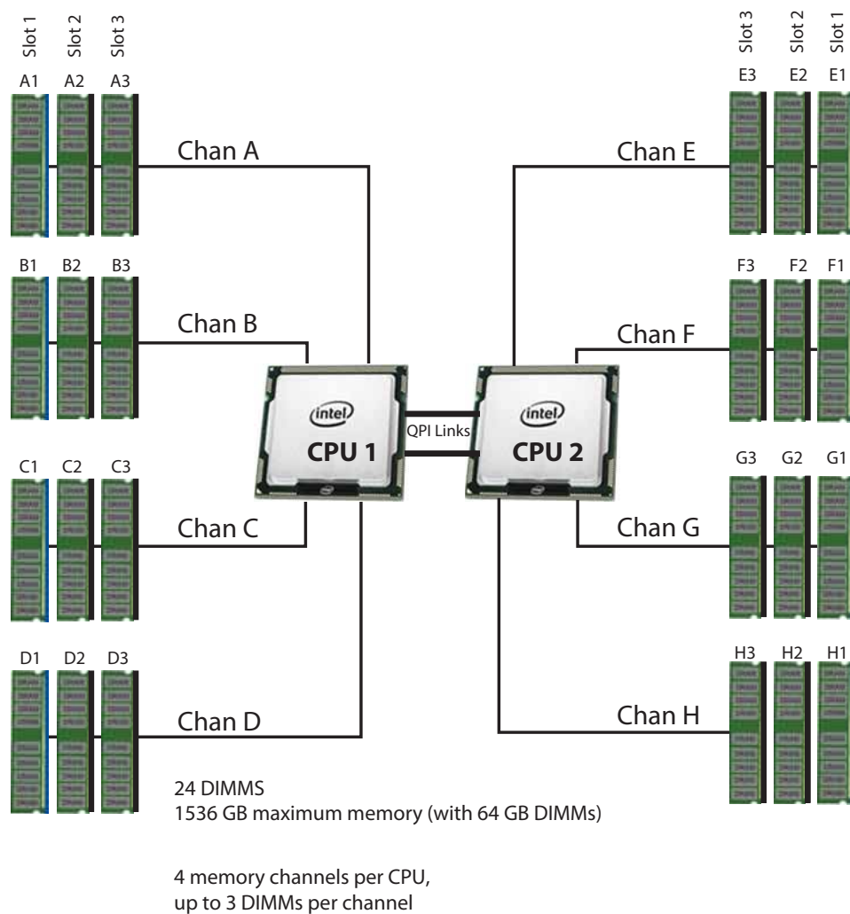
Figure 8 UCS B200 M4 Memory Organization
