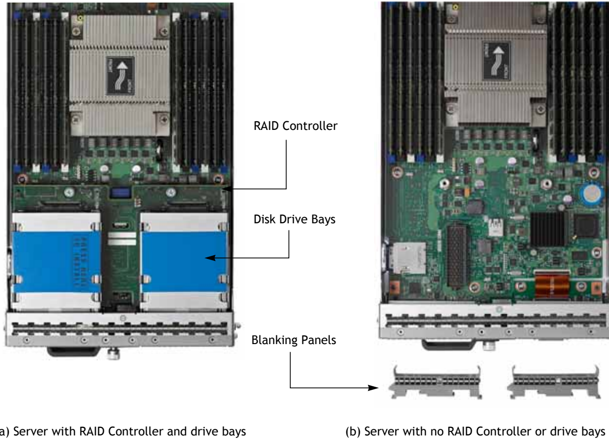
Figure 5 UCS B200 M4 With and Without RAID Controller (hidden) and Drives (Front View)
