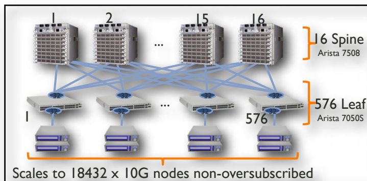
Arista Leaf-Spine Two-Tier Network Architecture
