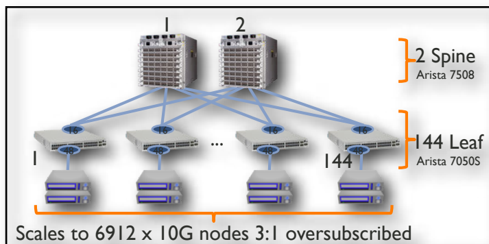
Arista Leaf-Spine Two-Tier Network Architecture
