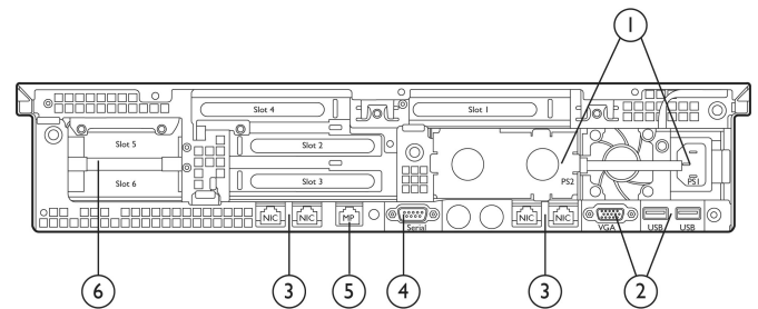
HP Integrity rx2800 i4 Server: Rear View
