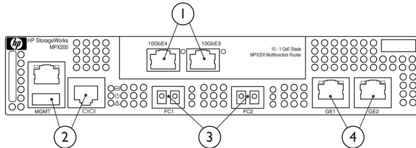
10GbE-1GbE blade shown in this picture
